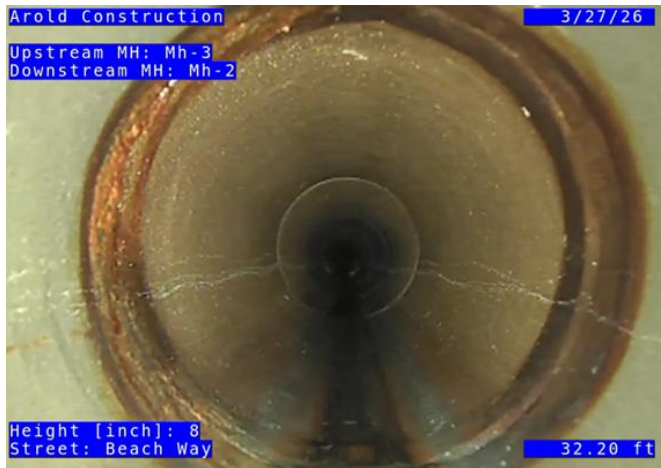
Inside View of Unlined Manhole and Sanitary Sewer Main
